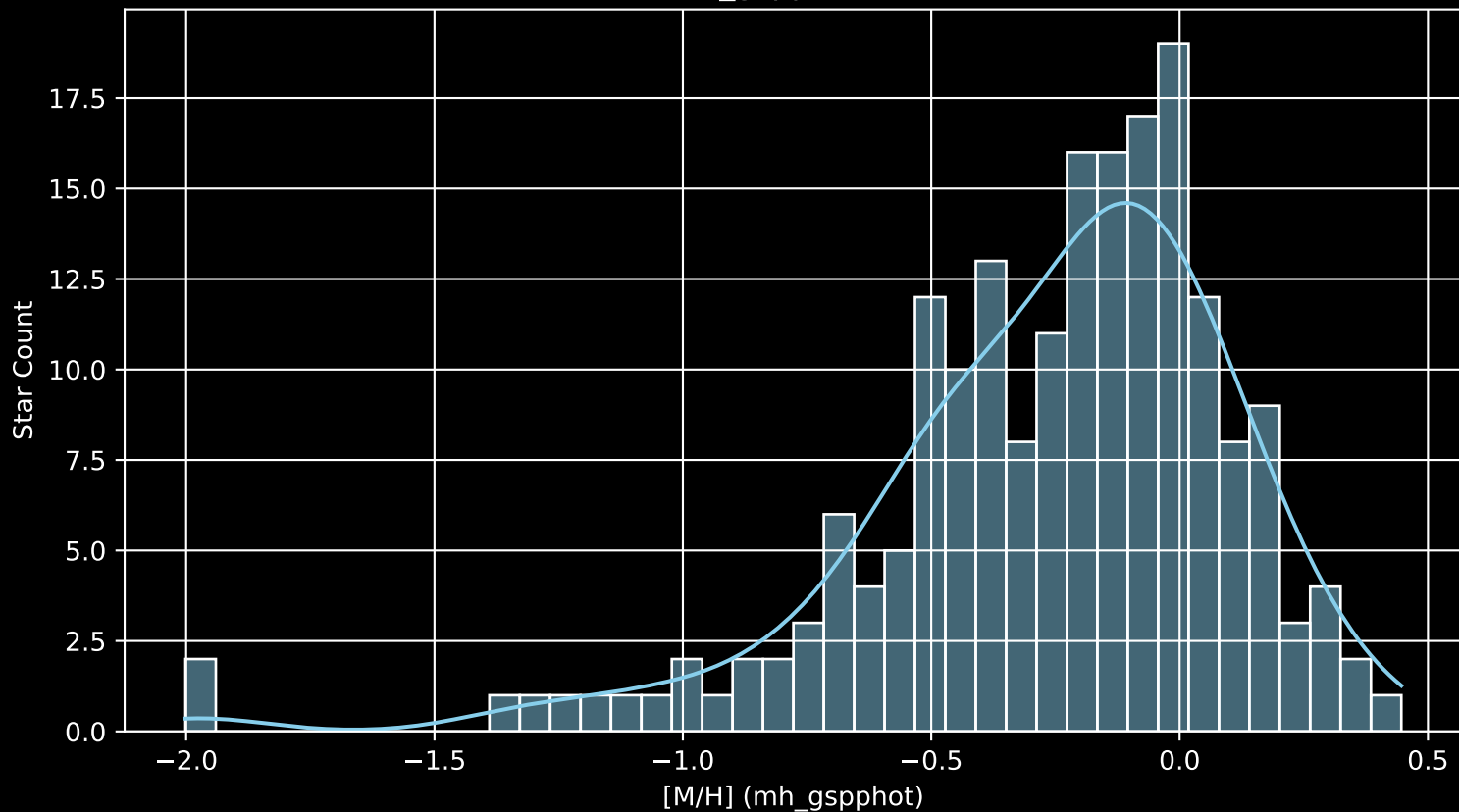
APOGEE DR17 Field: [LMC26 [M/H] (mh_gspphot) (n= 194)
