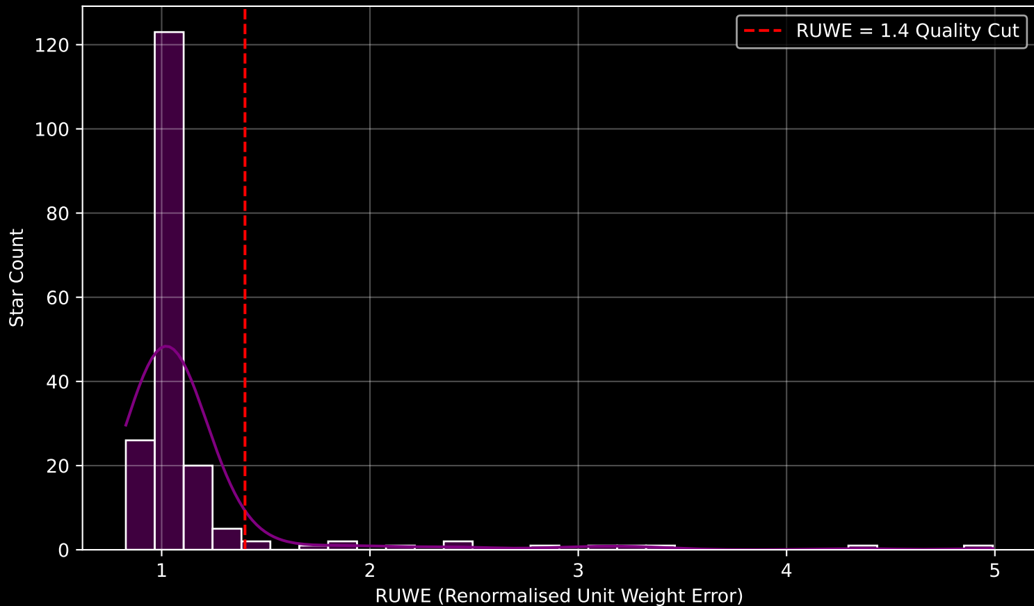
GAPOGEE DR17 Field [LMC26] RUWE Distribution (n= 188)
