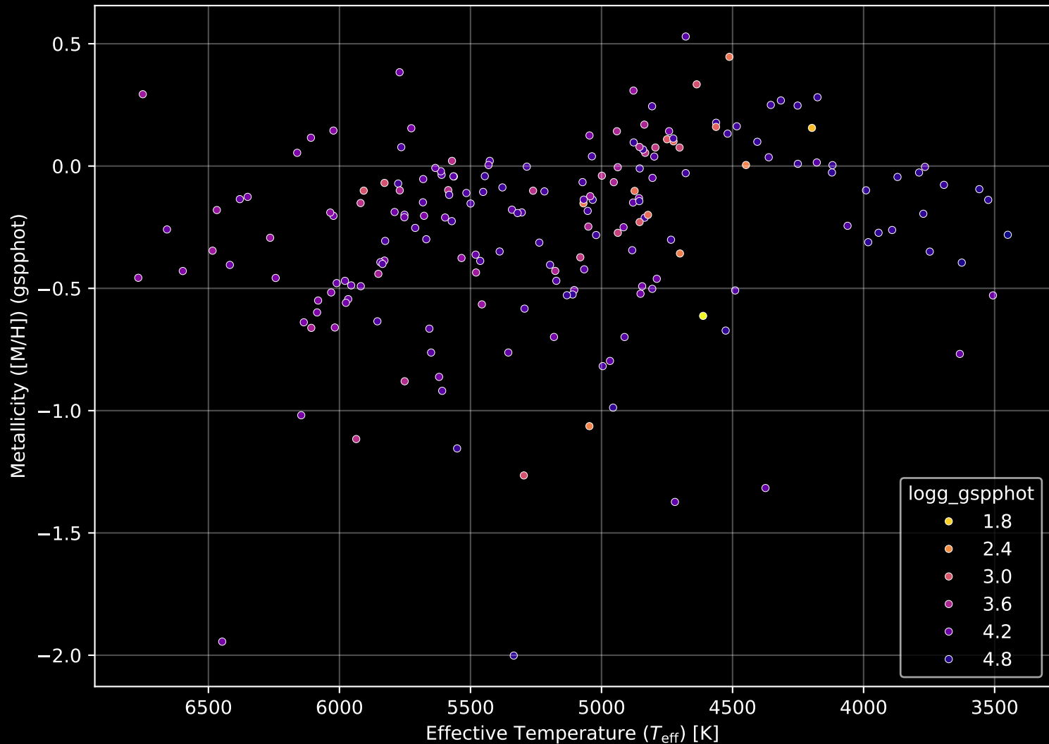
APOGEE DR17 Field: [LMC26] Stellar Population Parameters (n= 195)
