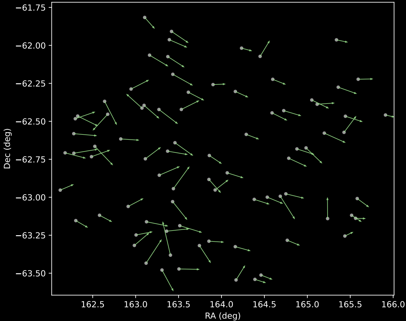
APOGEE DR17 Cluster 5 Proper Motion Vectors (n=81)
