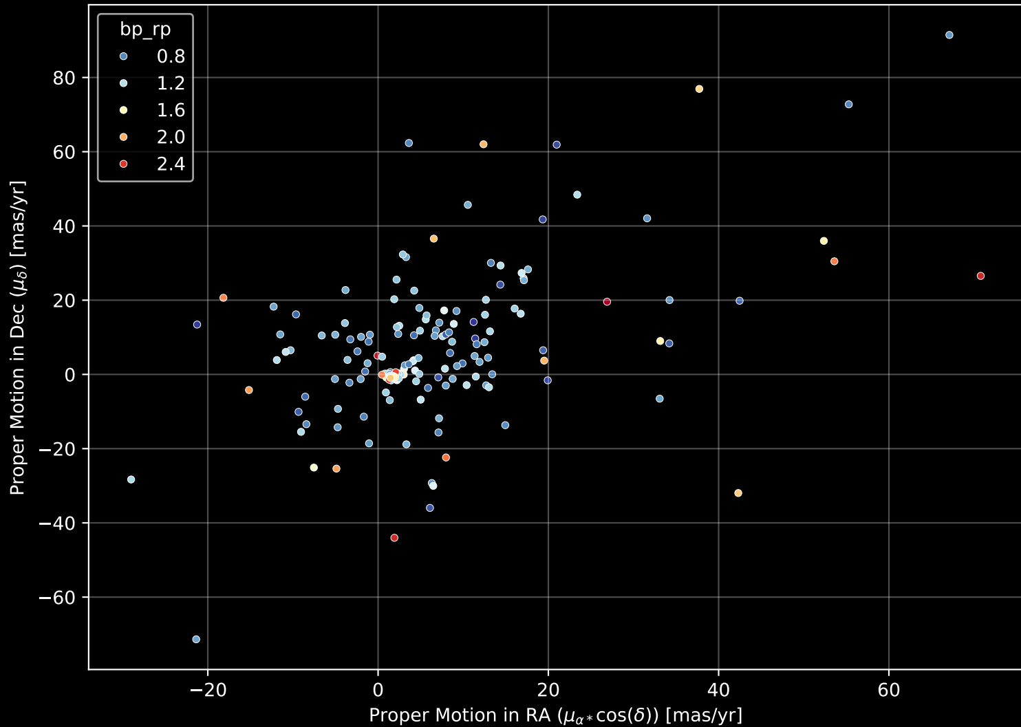
APOGEE DR17 Field: [LMC26] Proper Motion Diagram (n= 195)
