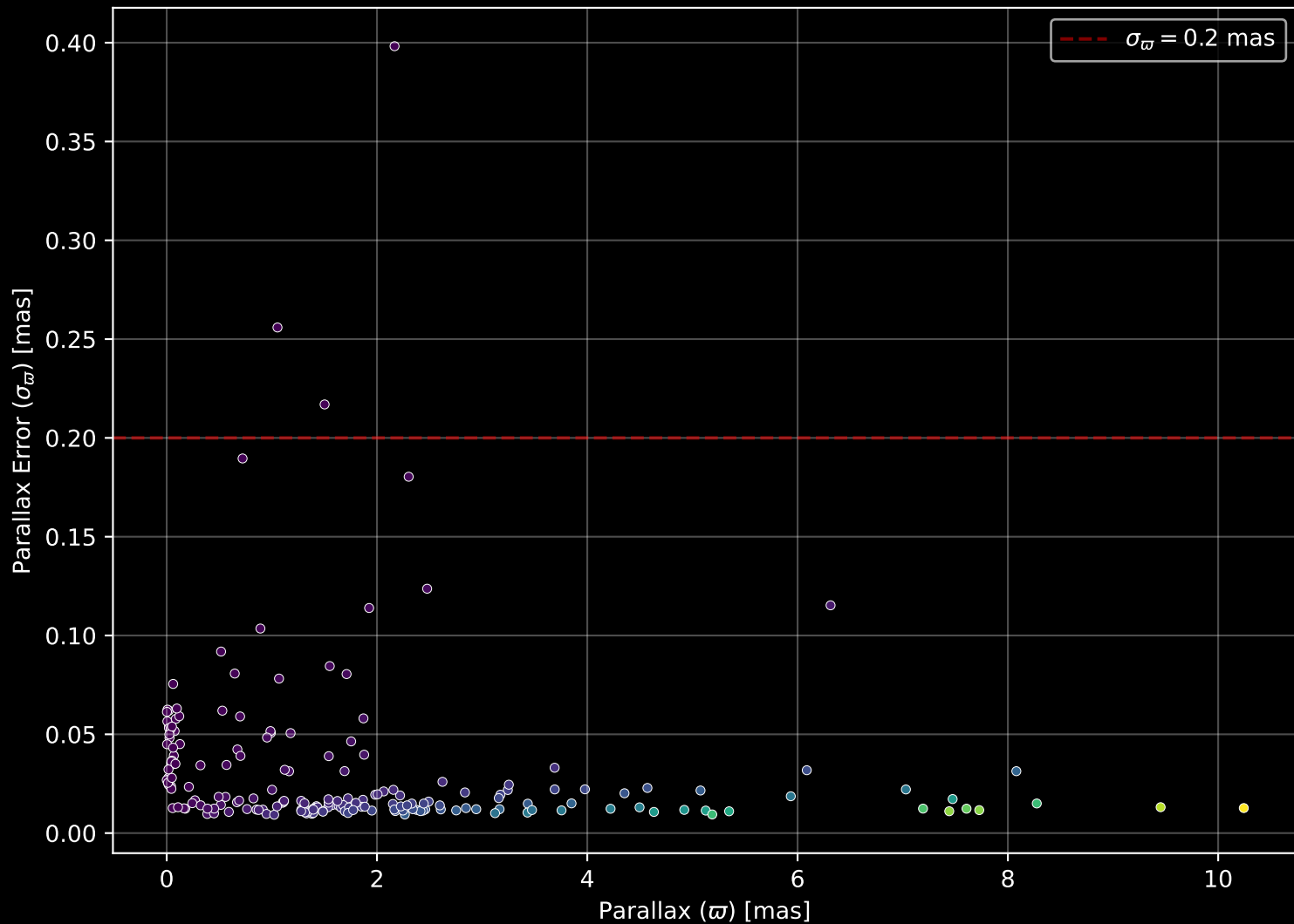
APOGEE DR17 Field: [LMC26] Parallax Quality (n= 195)
