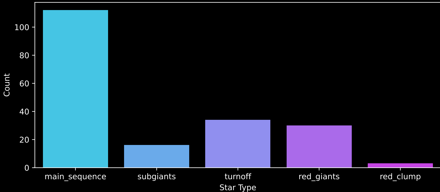
APOGEE DR17 Field: [LMC26] Count plot of Star Type
